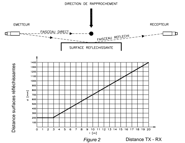
Figure 2 Distance TX - RX
